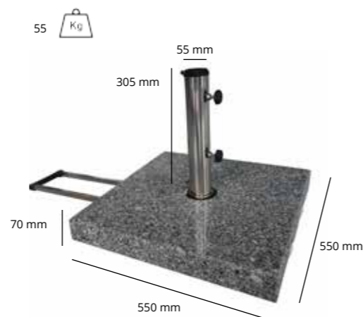
Base granite
