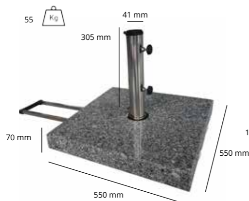
Base granite
